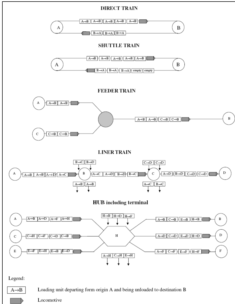
Fig.1 Alternative Rail Operating Forms
