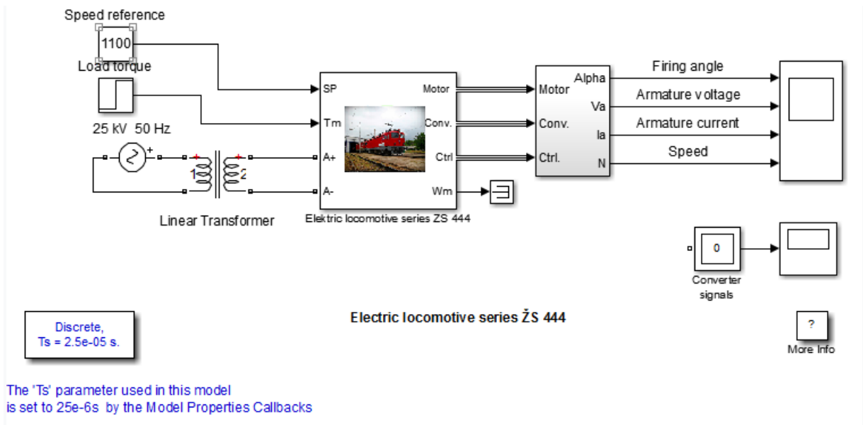
Fig. 3: Structural scheme of the model of the 444 series electric locomotive in Matlab-Simulink during speed control.
