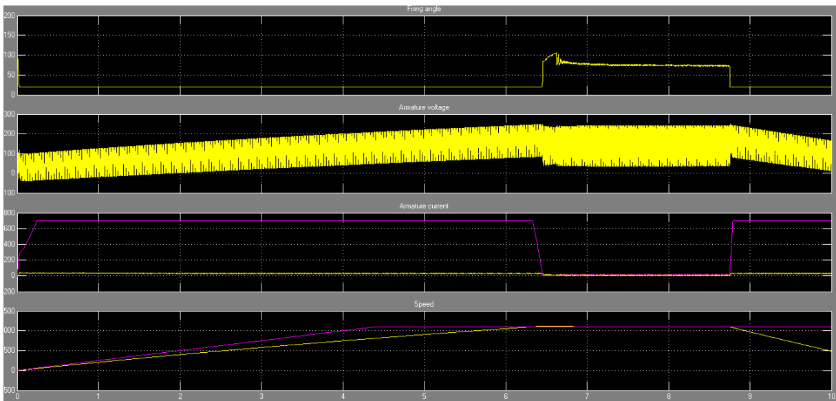
Fig. 15: Temporal changes of the ignition angle of the rectifier thyristor, voltage and armature current of the ŽS 444 locomotive electric motor in heavy freight trains
