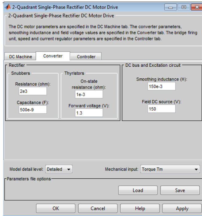
Fig. 10: Layout of the thyristor rectifier table dialog
