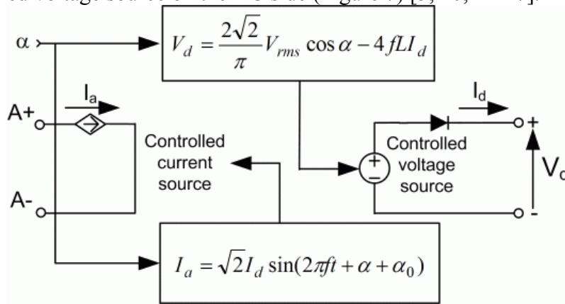
Fig. 7: Single-phase thyristor rectifier block
