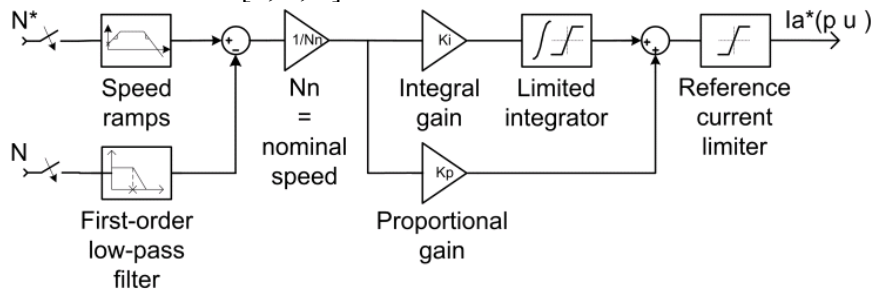
Fig. 5: Traction electric motor speed regulator block
