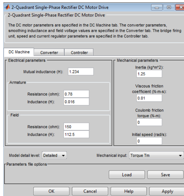
Fig. 9: Layout of the dialog table of the drive electric motor of direct current
