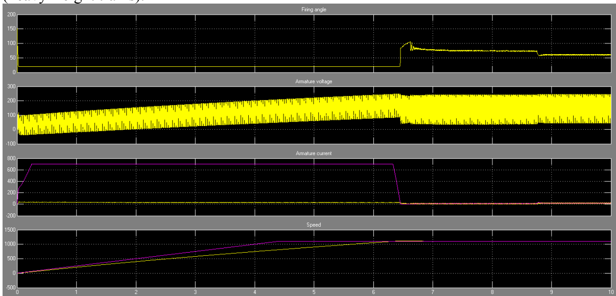
Fig. 14: Temporal changes of the ignition angle of the rectifier thyristor, voltage and armature current of the ŽS 444 series locomotive electric motor in light passenger trains
