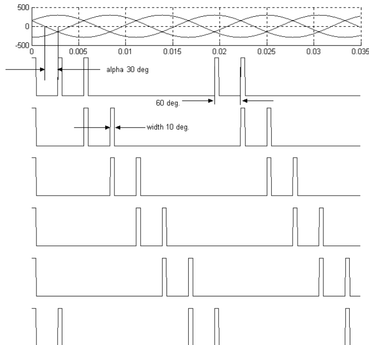
Fig. 8: Synchronized 6-pulse generator block configured in dual-pulse mode
