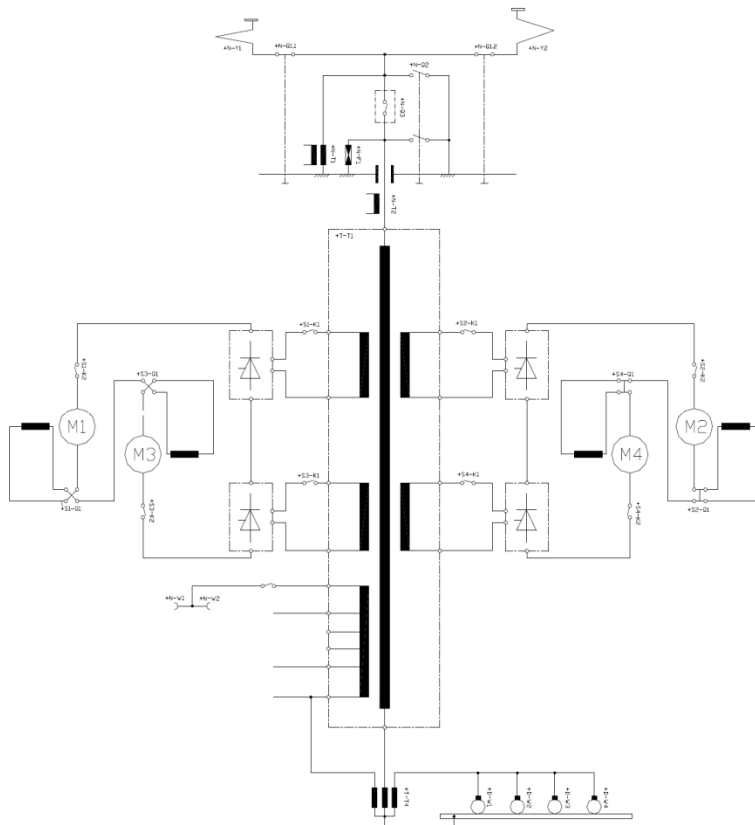
Fig. 2. Simplified diagram of the main circuit in traction [4]
