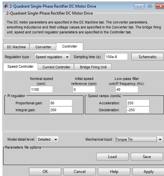
Fig. 11: Layout of the speed controller table dialog
