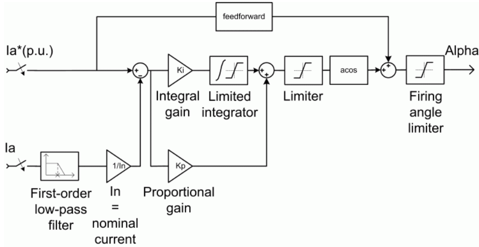
Fig. 6: Traction electric motor armature current regulator block
