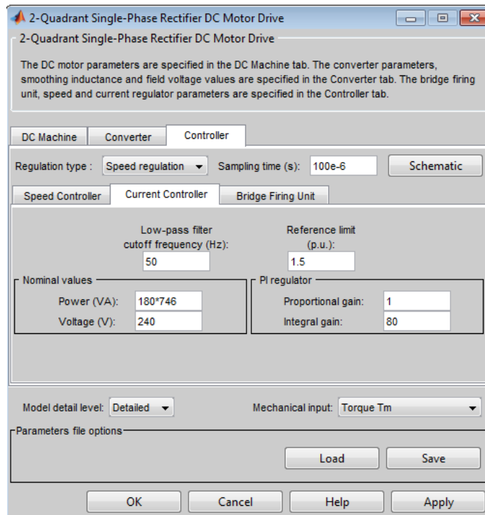
Fig. 12: Layout of the current controller table dialog
