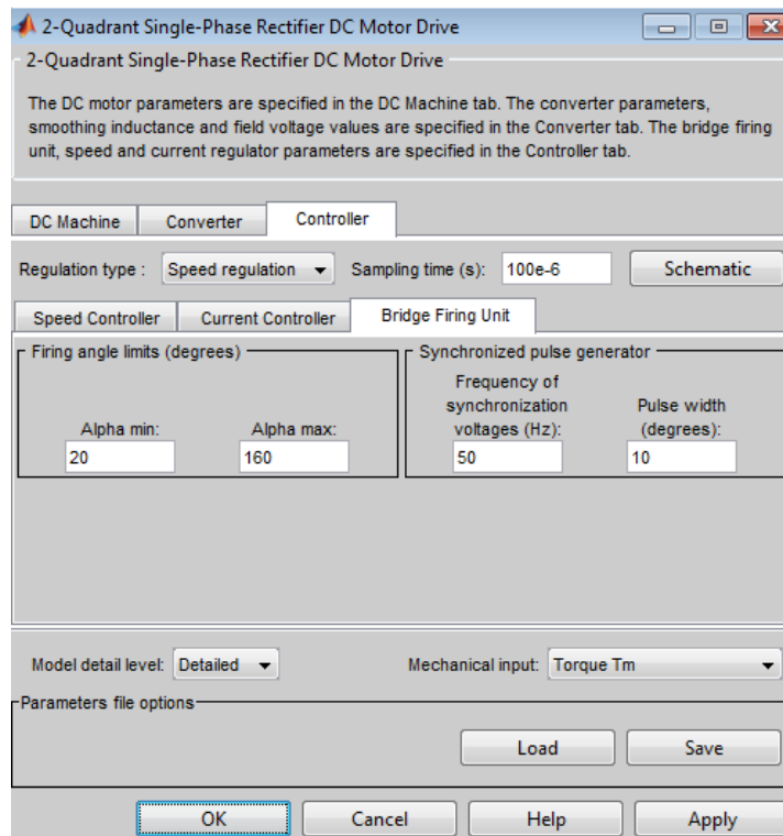
Fig. 13: Layout of the thyristor bridge ignition unit dialog
