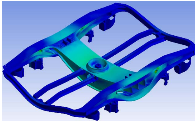
Fig. 12. FEM calculation of bogie frame
